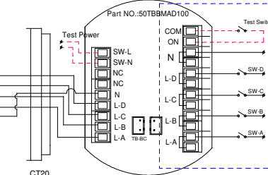
CT20 EXPLOSION CONNECTION
